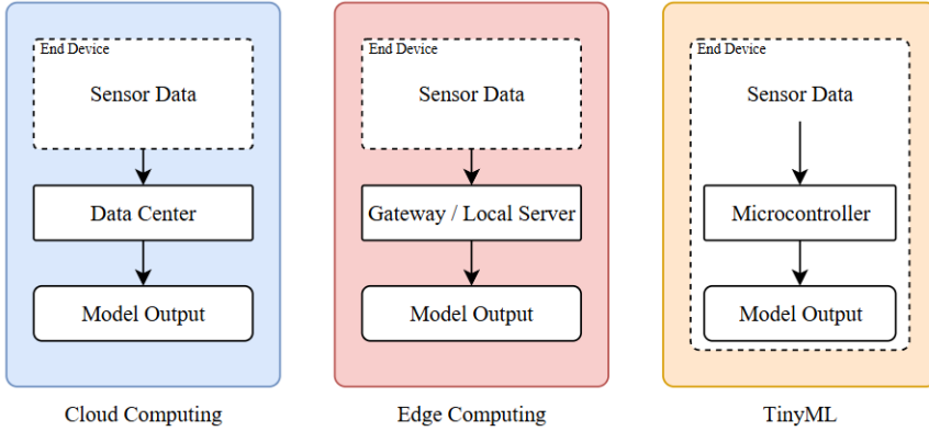
Figure 1. Inference locations and data flows in cloud computing, edge computing, and TinyML deployments.
