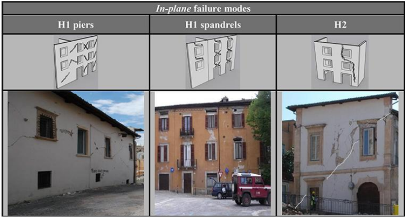
Figure 6: In plane failure modes
