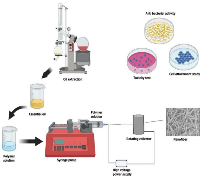
Figure 6: Schematic illustration an essential oil added electrospinning process
