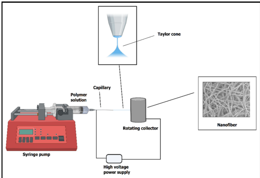
Figure 1: A schematic illustration of a basic electrospinning setup
