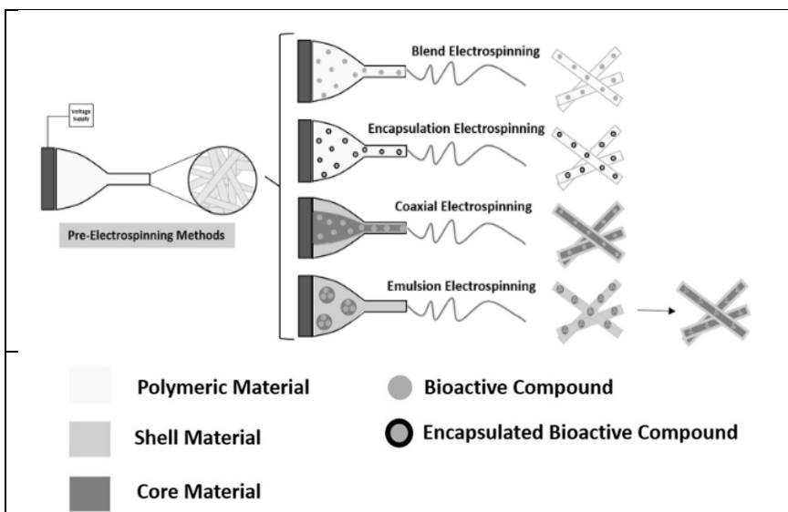
Figure 7: Schematic representation of the most common electrospinning techniques used for the incorporation of bioactive compounds into nanofibers
