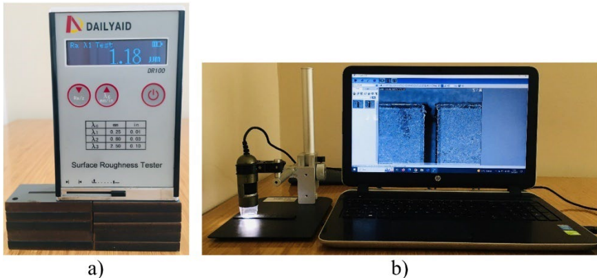
Figure 1. Devices used for measuring responses: (a) Surface roughness tester; (b) Digital microscope
