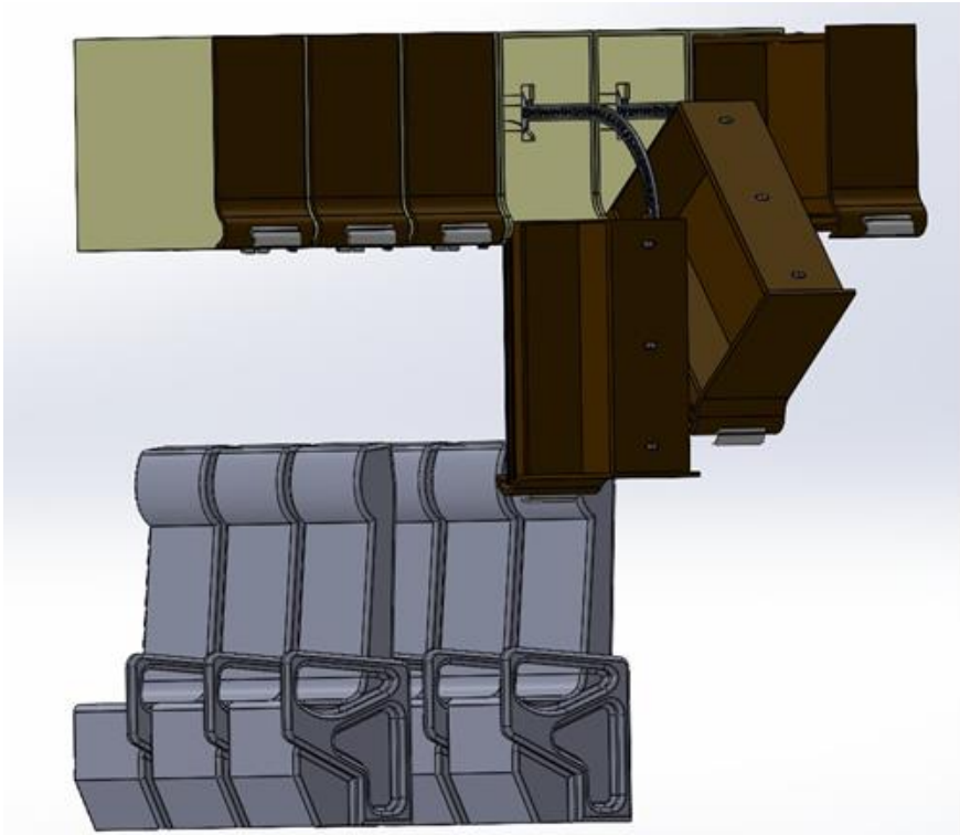
Figure 3 - Depicting the arrangement of seats and storage compartments
