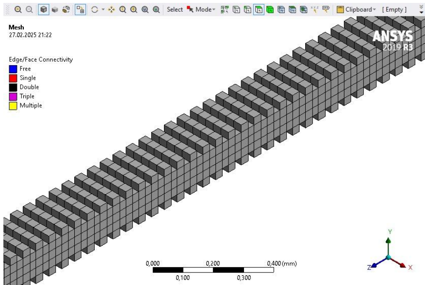
Figure 4 Mesh view
