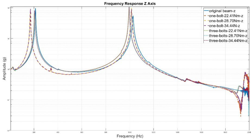
Figure 6: Transfer function of z direction-analysis
