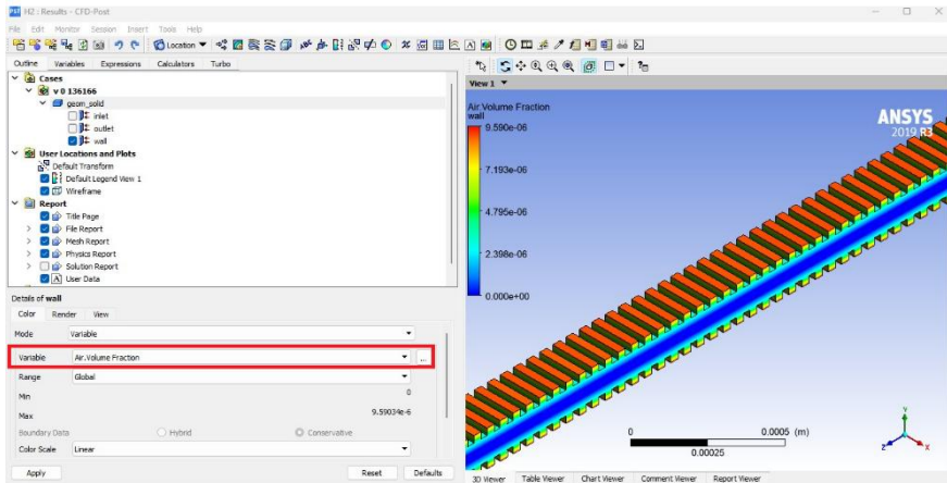
Figure 13 Air volume fraction images ( d = 28 \mu\text{m} a = 32 \mu\text{m} h=30\mu\text{m} )
