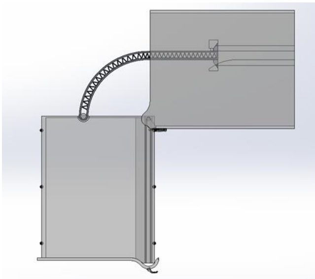
Figure 2-Side view of the cabin storage system design
