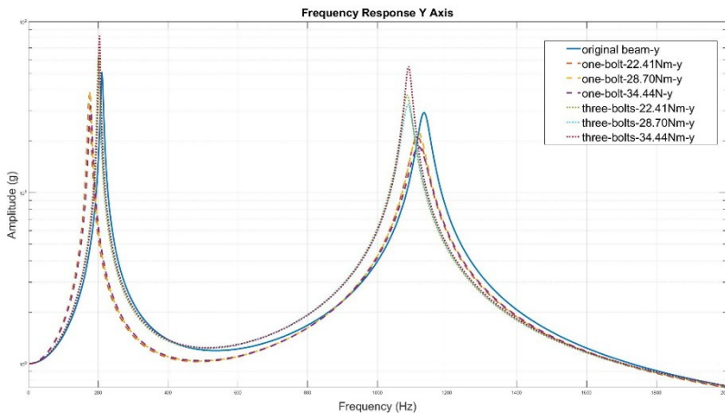
Figure 4 Transfer function of y direction-analysis
