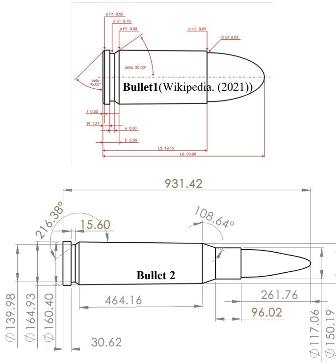
Figure 1. Dimensions of designed plate and bullets
