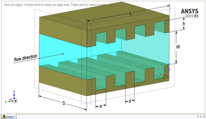
Figure 3 Design of microchannel
