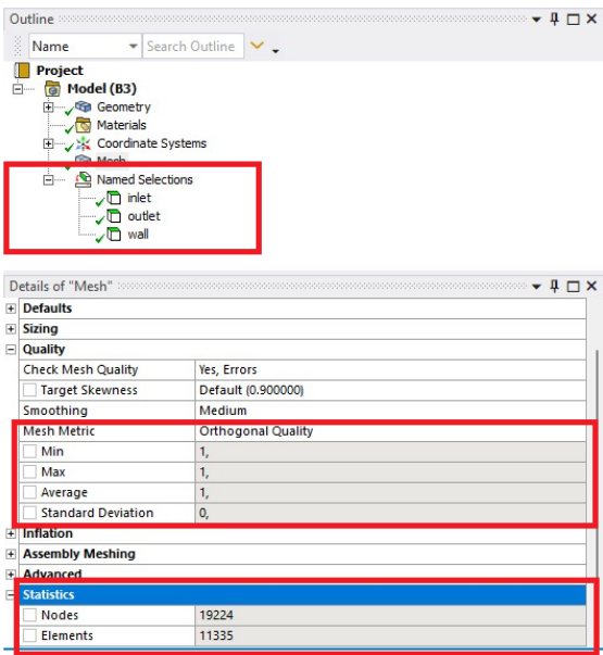
Figure 5 Mesh information
