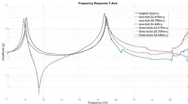
Figure 3 Transfer function of y direction-test
