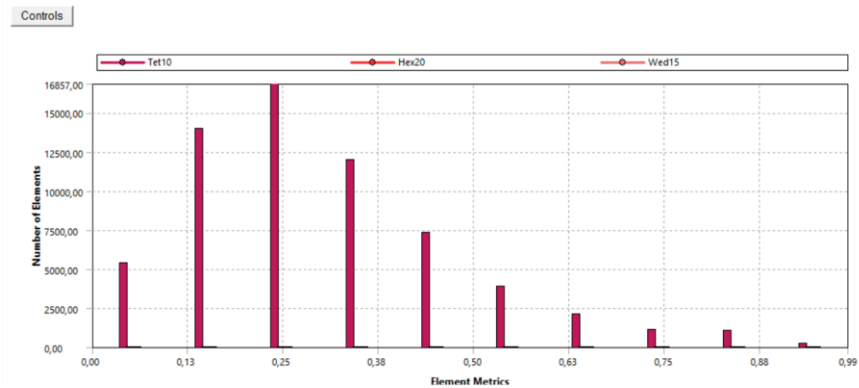
Figure 7 - Mesh quality (Skewness)
