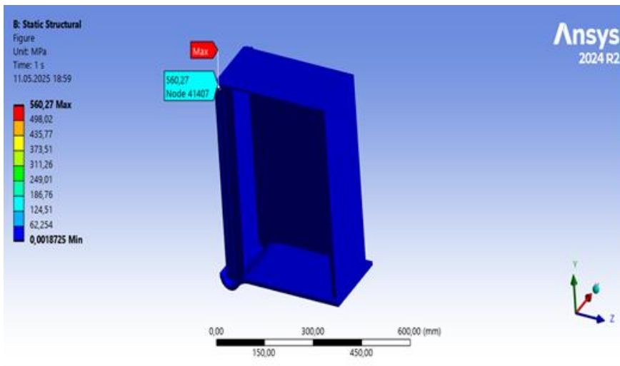
Figure 9 - Von mises stress
