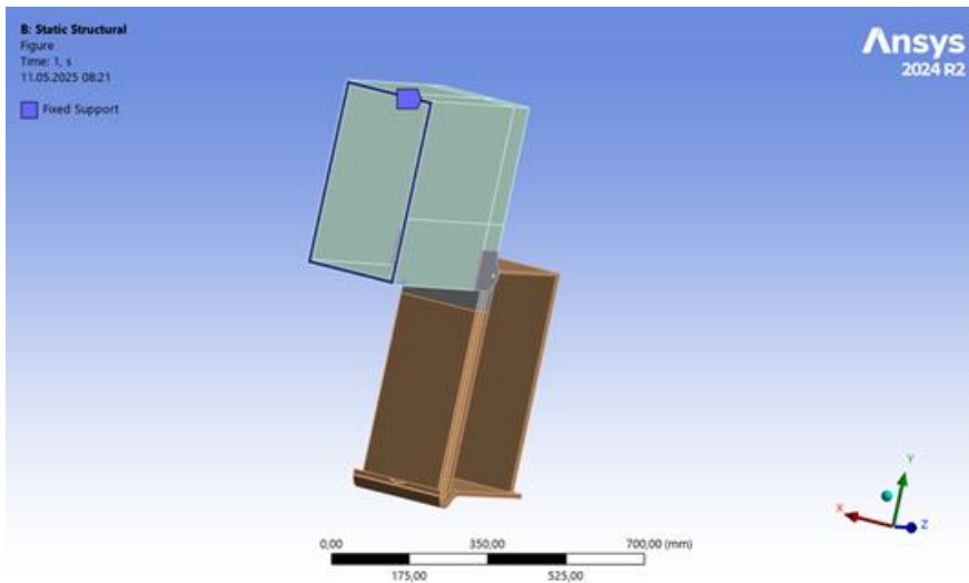
Figure 4 - Boundary condition
