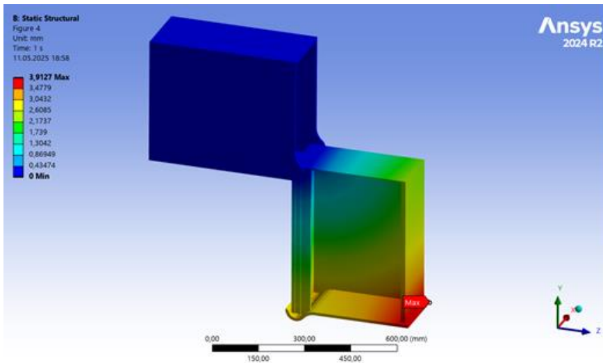
Figure 8 - Total deformation
