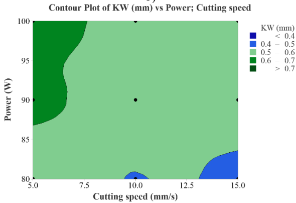
Figure 3. Contour plots for KW: a) Material type–Power, b) Material type–Cutting speed, and c) Power–Cutting speed
