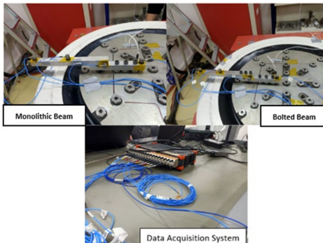
Figure 2 Data acquisition system and configuration of beams
