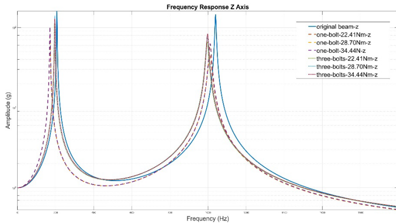
Figure 6: Transfer function of z direction-analysis
