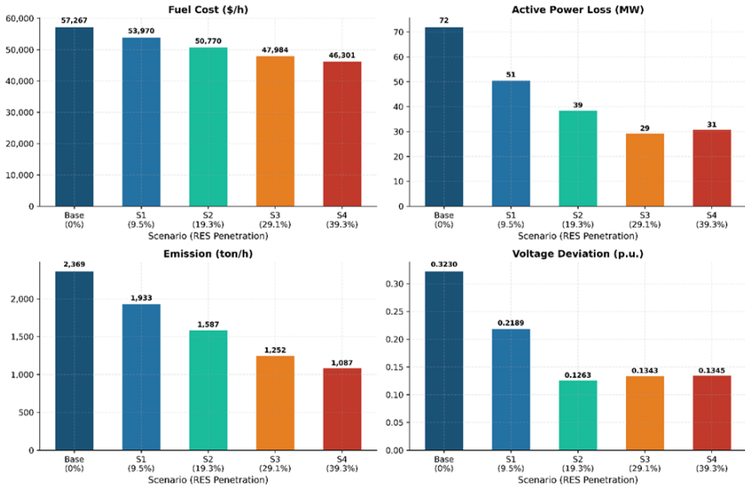
Figure 3: Bar charts of f_1, f_2, f_3, f_4 across Base, S1–S4 for HLWOA best compromise solution.
