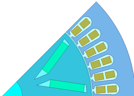
Figure. 1 Machine topology.
