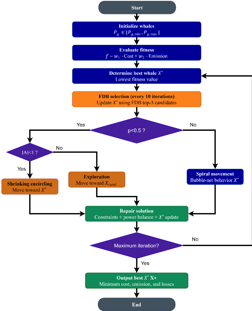
Figure 4 FDB-WOA Flow Diagram
