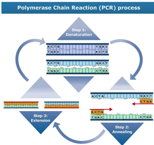
Figure 4. Polymerase Chain Reaction Process
