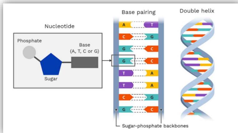
Figure 1. The structure of DNA
