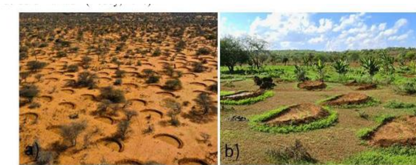
Figure 4. Examples of semicircular earthen bunds in Kenya: (a) Naibunga Conservancy, Kenya; (b) Olorika region, Kenya
