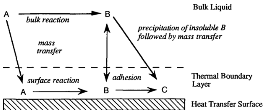
Figure 9: General diagram of the chemical reaction contamination mechanism
